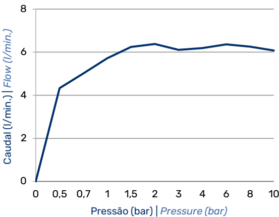
DIAGRAMA CAUDAL | FLOW DIAGRAM
