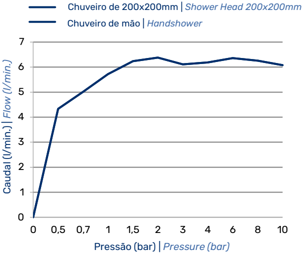
DIAGRAMA CAUDAL | FLOW DIAGRAM
